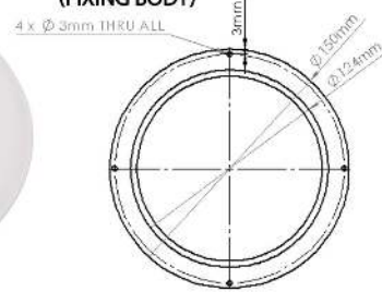
BACK VIEW (FIXING BODY)
