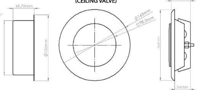
FRONT VIEW (CEILING VALVE)
